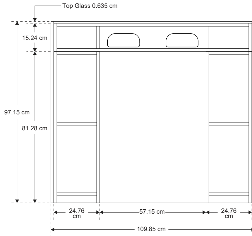
Single Unit Front View
