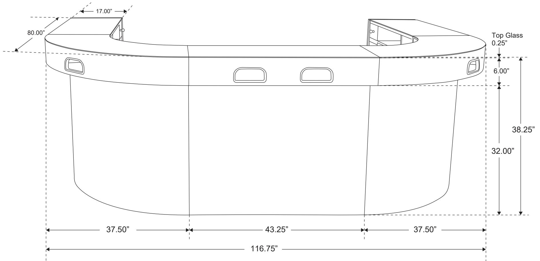
5-Person "U" Shape Nail Bar
