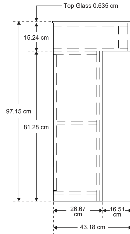
Single Unit Side View
