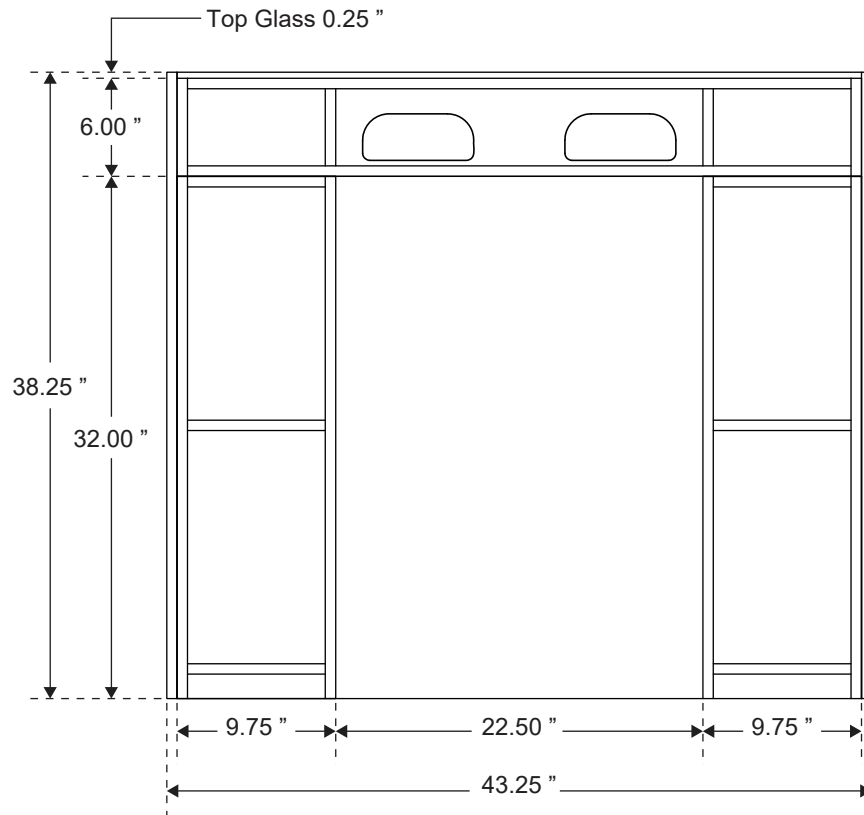
Single Unit Front View
